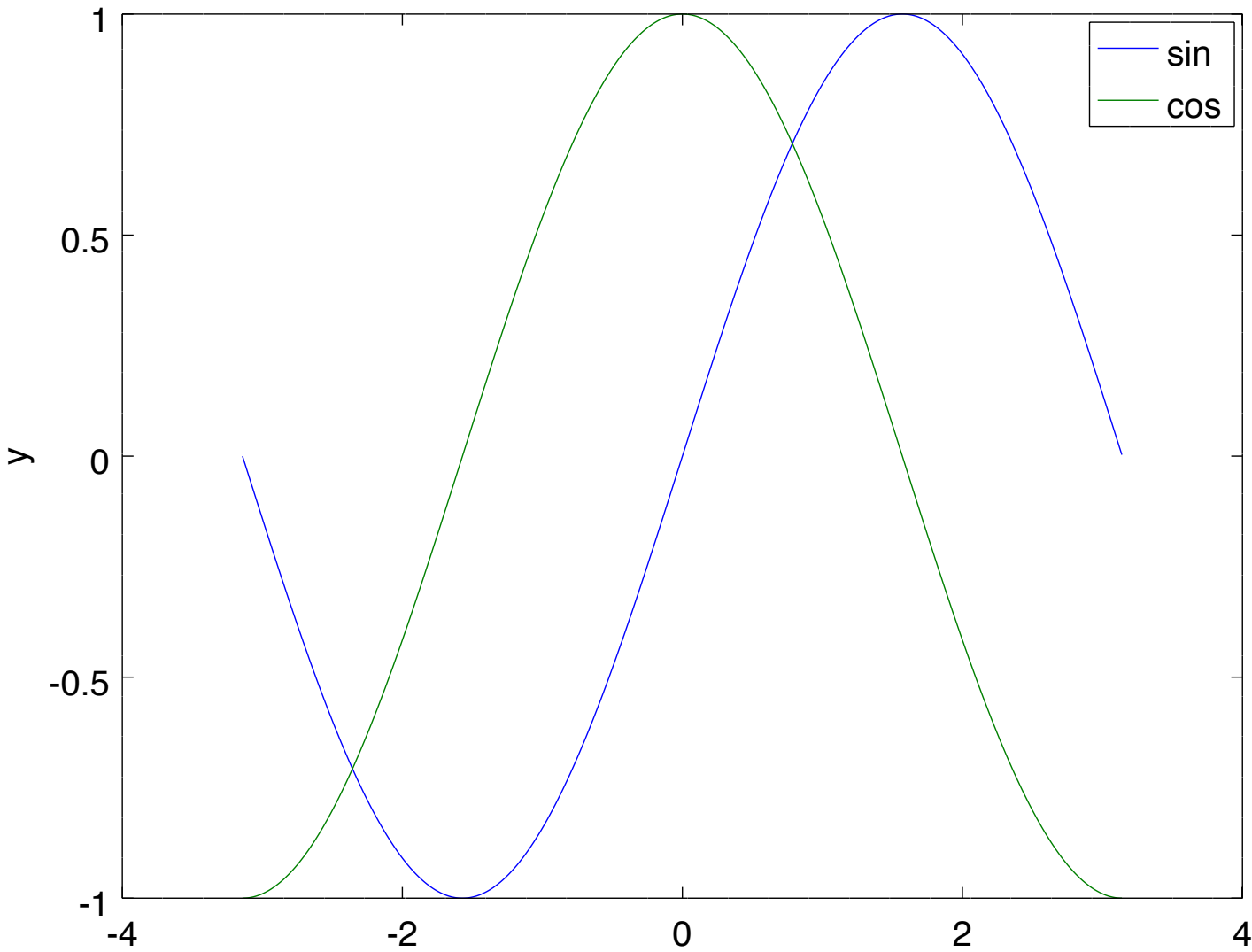
sin and cos
